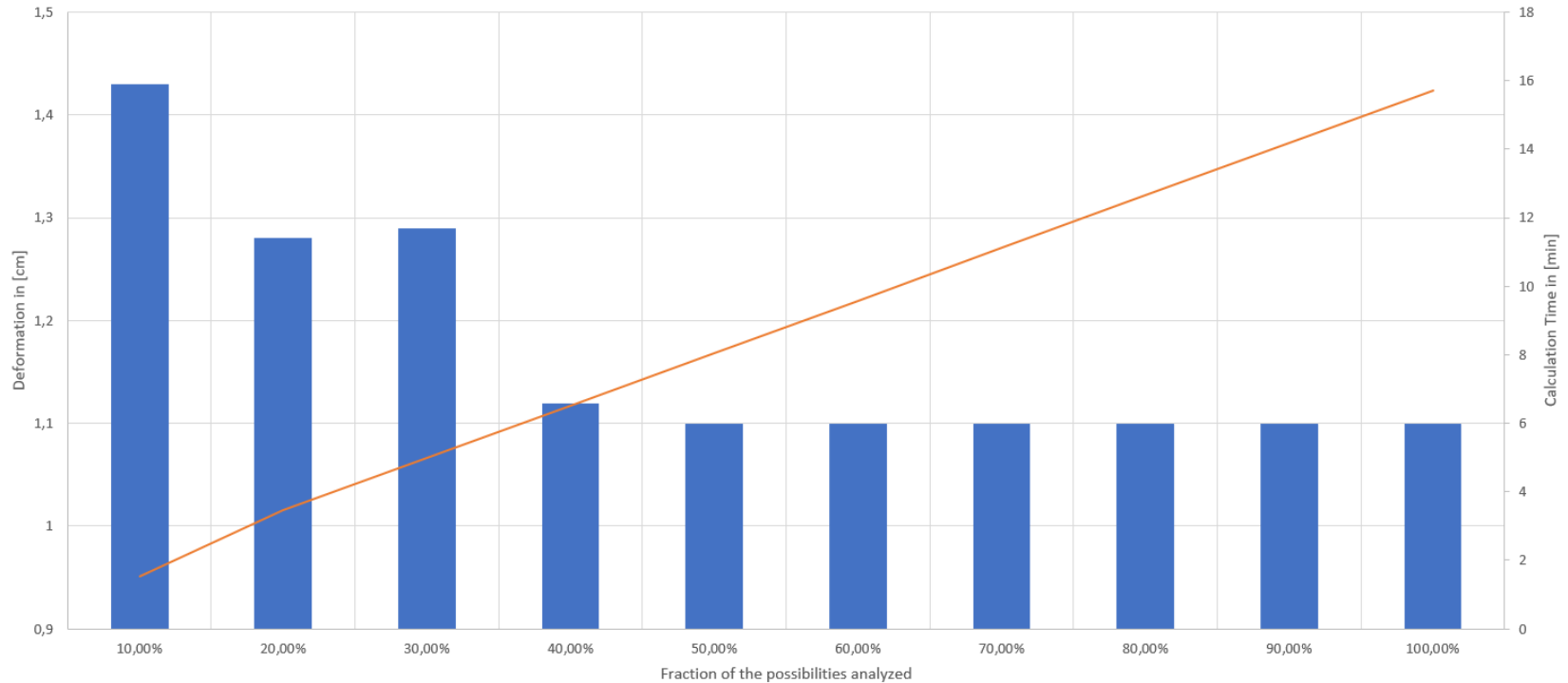
Optimization of global parameters
